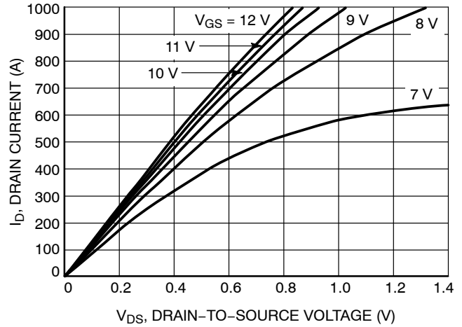
Figure 4. Saturation Characteristics
