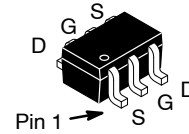
SC-88/SC70-6/SOT-363 CASE 419B-02
