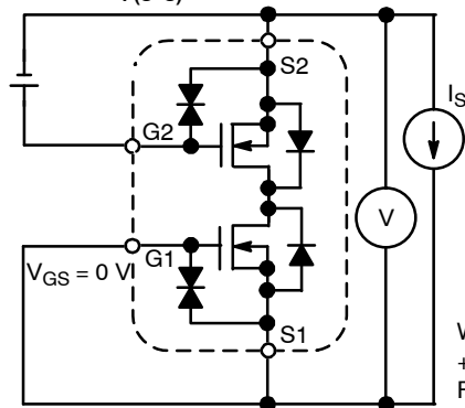
Test Circuit 7
