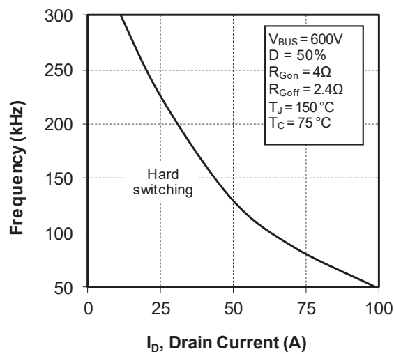
Figure 1-28. Operating Frequency vs. Drain Current
