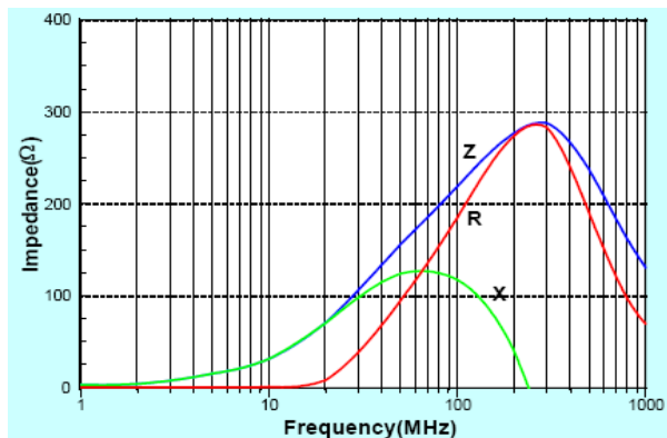
ACML-0805U-221
