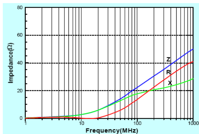
ACML-0805U-220
