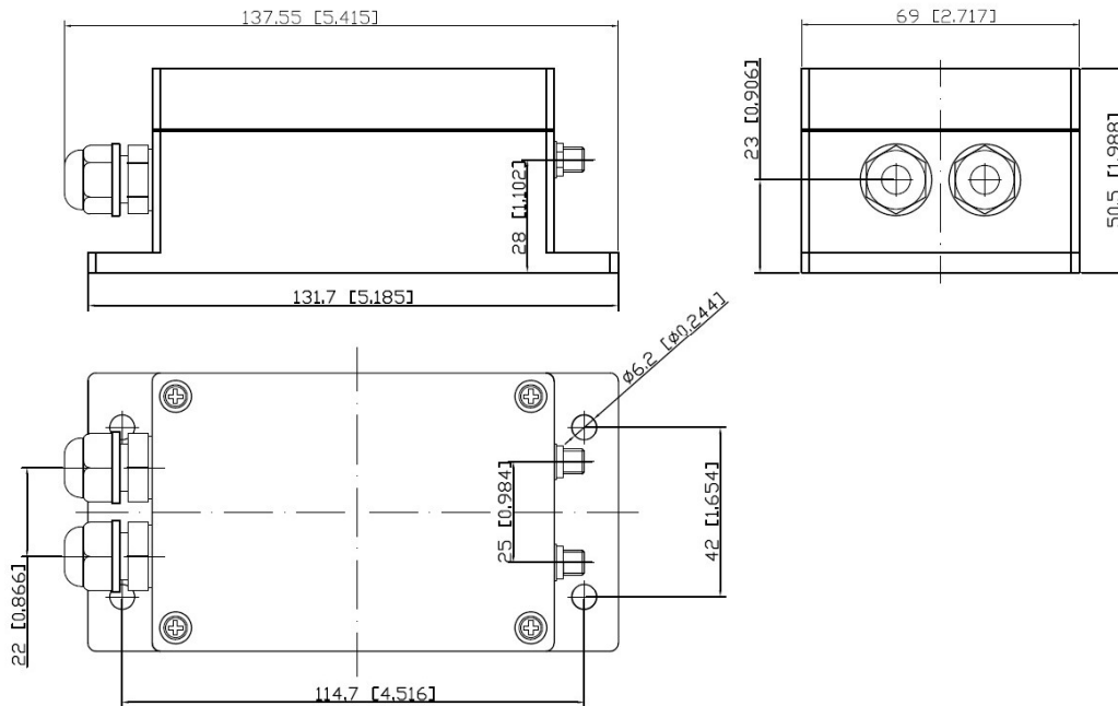
Pic. 6. qBox Enclosure Plus Kit (Two SMA) dimensions
