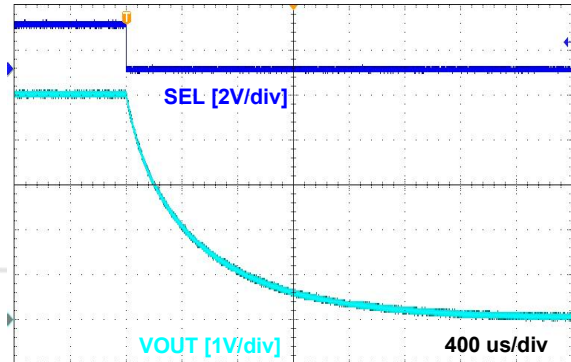
Figure 15. Turn-Off Response
