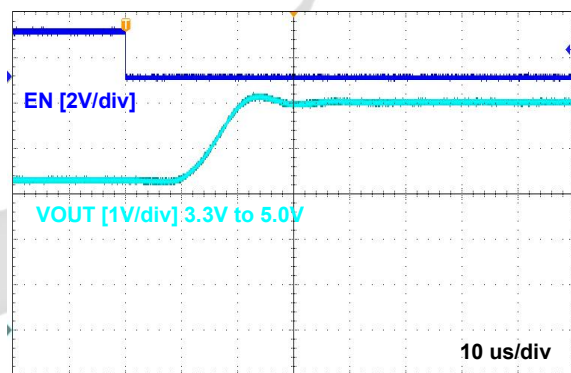
Figure 17. V_{OUT} Switchover 3.3 V_{IN} to 5 V_{IN}
