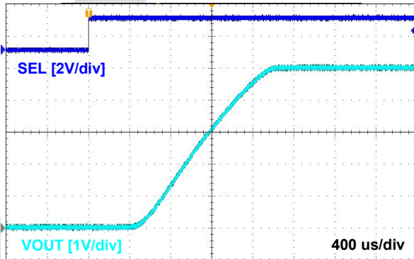
Figure 14. Turn-On Response
