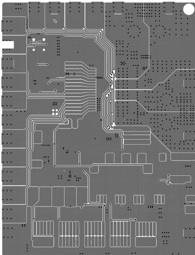
Figure 8. Bottom Layers
