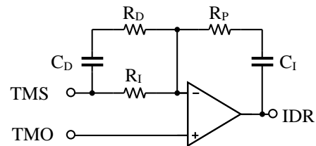
Figure 13. Compensation network
