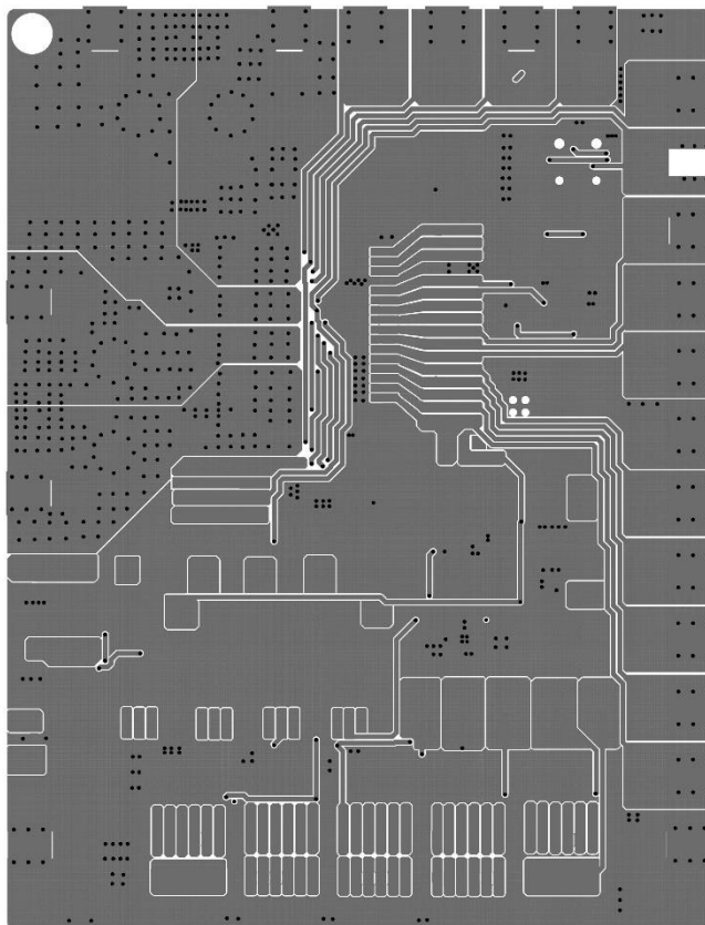
Figure 9. Mirrored Bottom Layers
