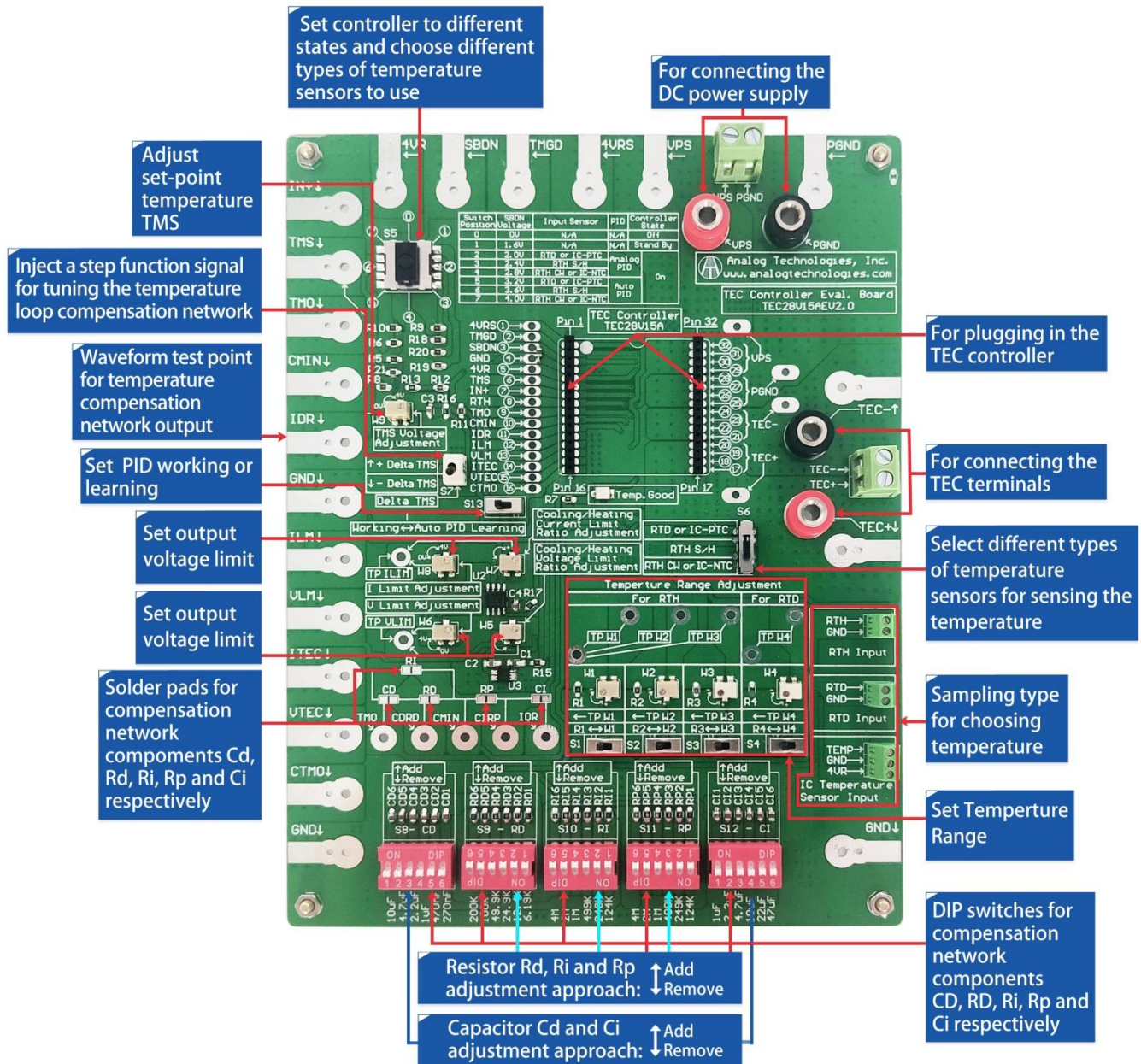
Figure 3. Board Description
