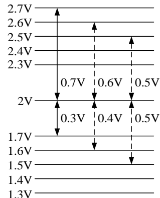
Figure 16. Adjust W7 or W5
