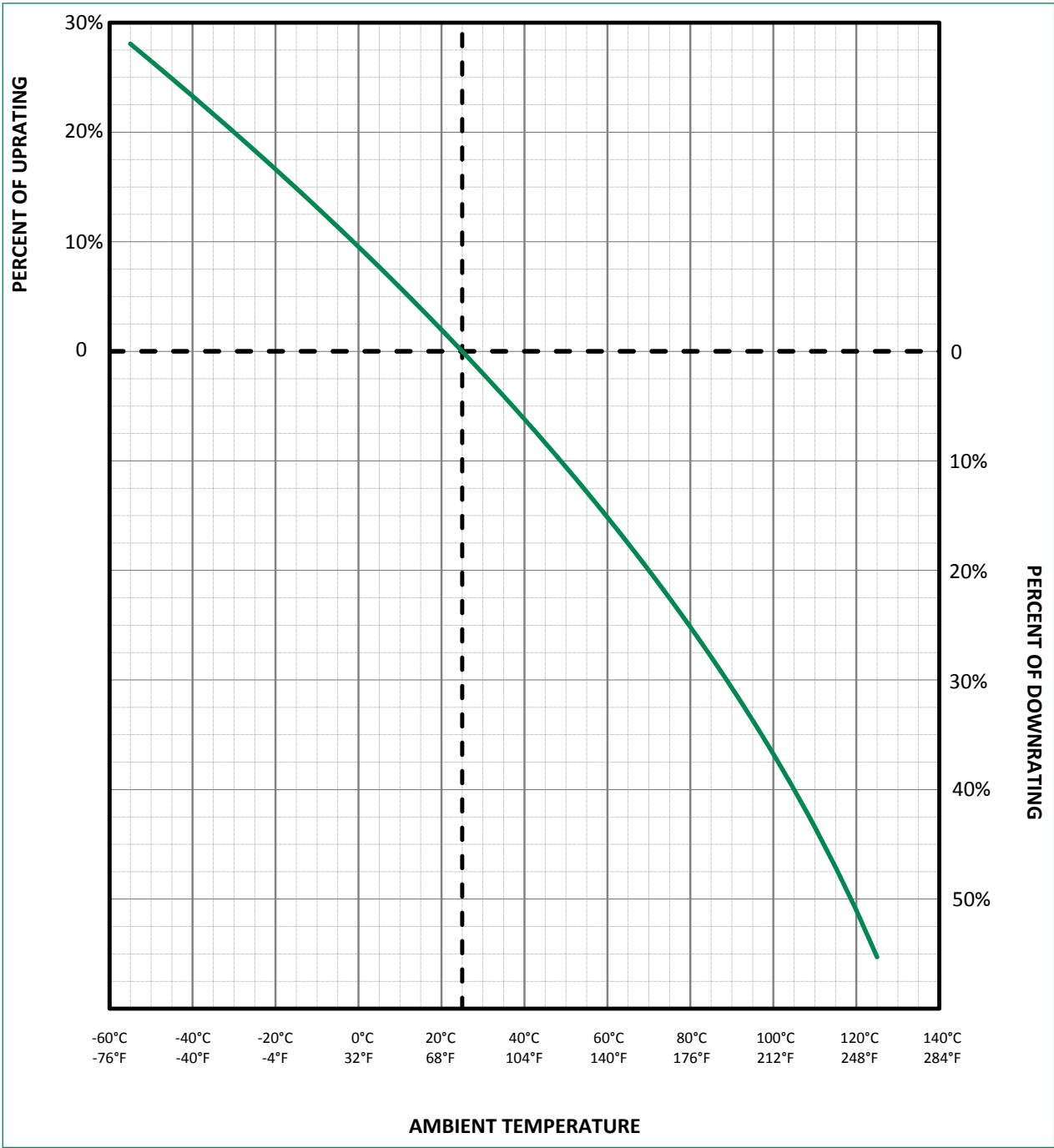
Temperature De-rating Curve (temperature of air immediately surrounding fuse) L75QS Series
