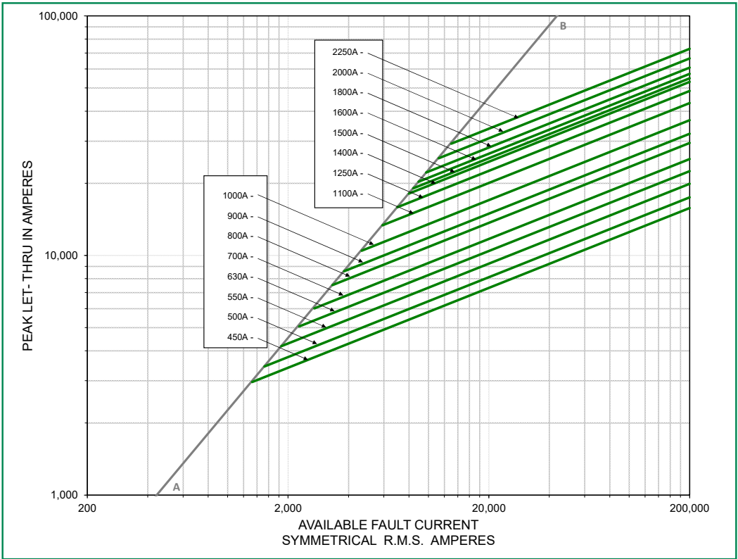
Peak Let-Thru Curve (33 Case Size)
