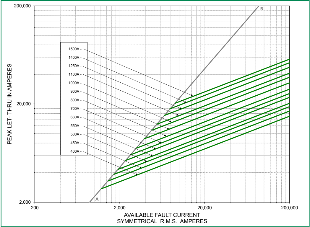
Peak Let-Thru Curve (32 Case Size)
