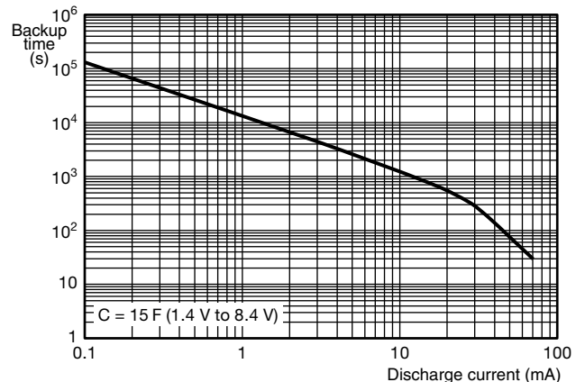
Fig. 19 - Typical Backup Time as a Function of Discharge Current
