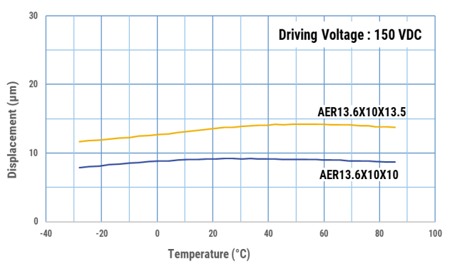
Figure 3 - Temperature vs. Displacement
