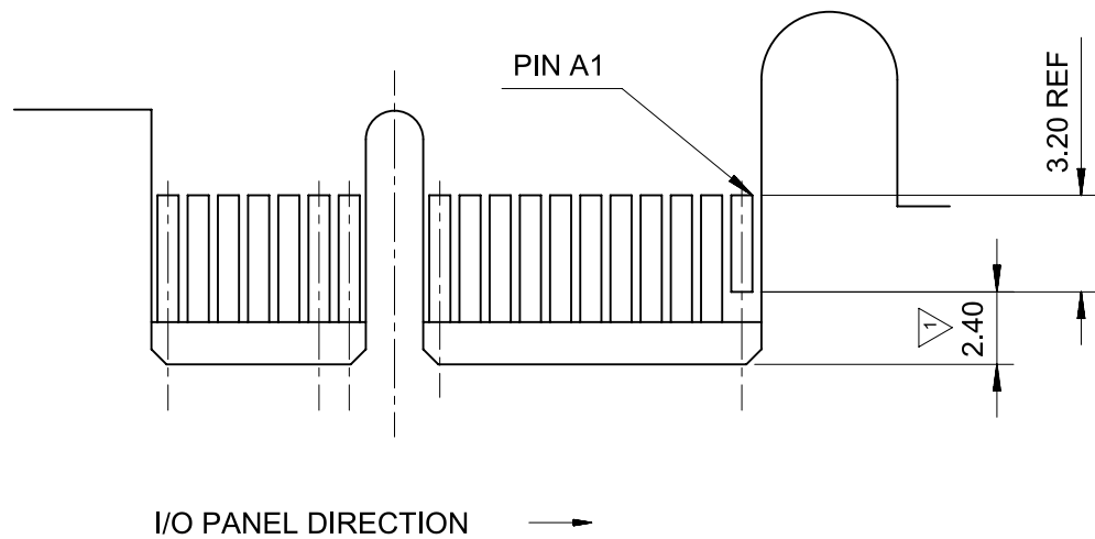
SECONDARY (SOLDER) SIDE
