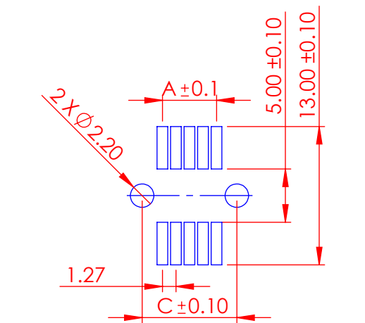
RECOMMENDED PCB LAYOUT (CONTACT CODE 99, MOUNTING CODE 05)
