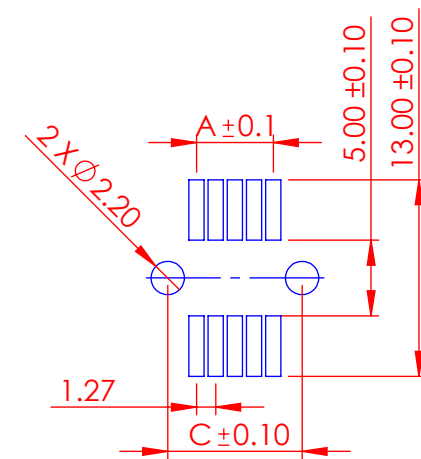
RECOMMENDED PCB LAYOUT (CONTACT CODE 99, MOUNTING CODE 05)
