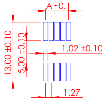
RECOMMENDED PCB LAYOUT (CONTACT CODE 99, MOUNTING CODE 01)
