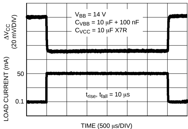
Figure 7. Load Transient Response ( I_{CC} 100 \mu A to 50 mA)
