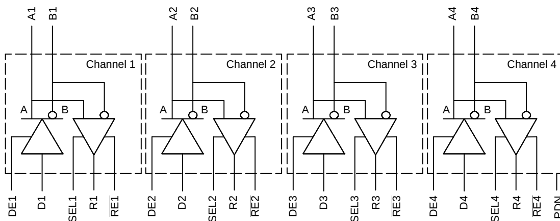
Figure 2. Block Diagram
