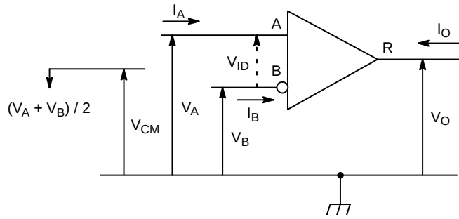
Figure 3. Receiver Voltage and Current Definitions
