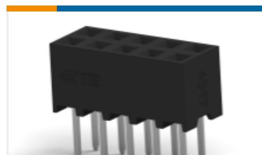
TE Part # 1-2314812-0 10P,2MM,B-B,REC,DRVT,2.0,0.1AU,TB, W/CAP
