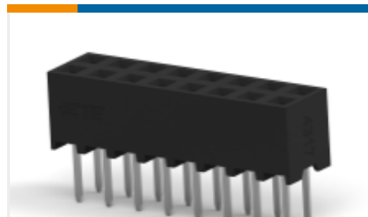
TE Part # 1-2314811-6 16P,2MM,B-B,REC,DRVT,2.0,SN,TB W /CAP
