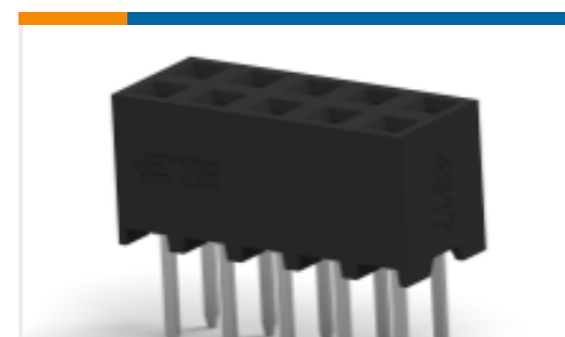
TE Part # 1-2314814-0 10P,2MM,B-B,REC,DRVT,2.0,0.76AU, TB,W/CAP
