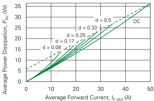
Figure 5. Forward Power Loss Characteristics
