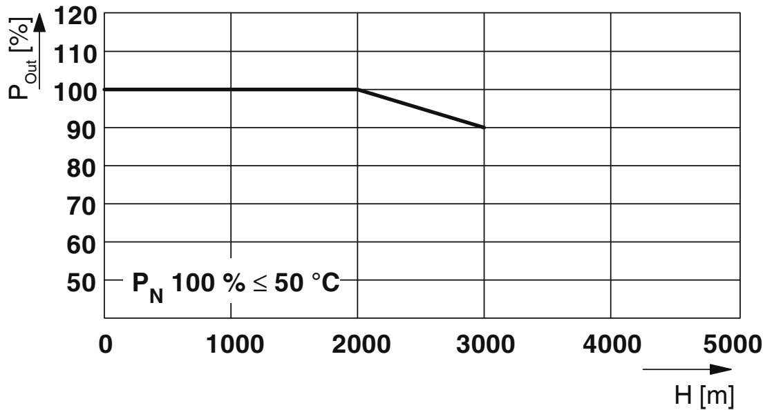
Altitude-dependent derating
