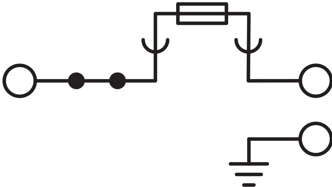
Circuit diagram
