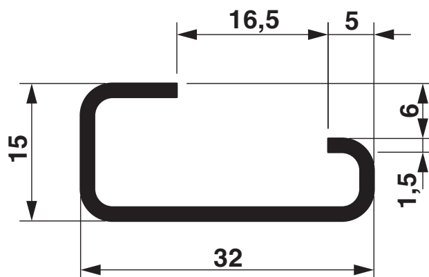
Dimensional drawing
