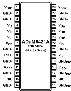
Figure 4. ADuM6421A Pin Configuration
