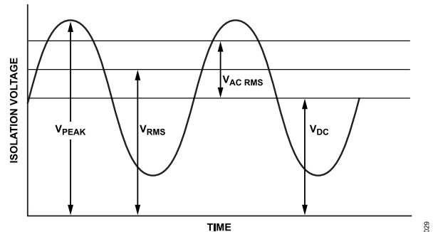
Figure 27. Critical Voltage Example
