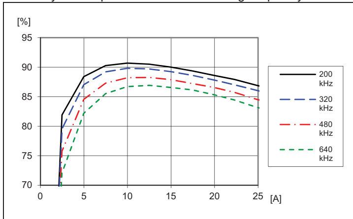
Efficiency vs. load current and switching frequency at T_{P1} = +25\text{ }^{\circ}\text{C} , V_I = 12\text{ V} , V_O = 1.0\text{ V} , C_O = 470\text{ }\mu\text{F}/10\text{ m}\Omega . Default configuration except changed frequency
