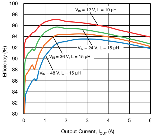
Fig. 23 - SiC473 Efficiency vs. Output Current, VOUT = 5 V
