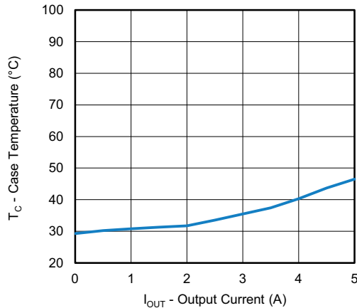
Fig. 25 - SiC473 Load Current vs. Case Temperature, VIN = 48 V, VOUT = 5 V
