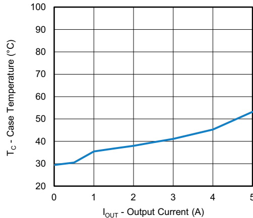
Fig. 28 - SiC473 Load Current vs. Case Temperature, VIN = 48 V, VOUT = 12 V
