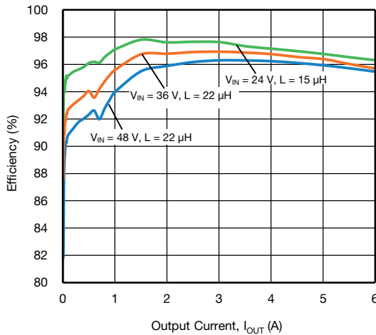
Fig. 24 - SiC473 Efficiency vs. Output Current, VOUT = 12 V
