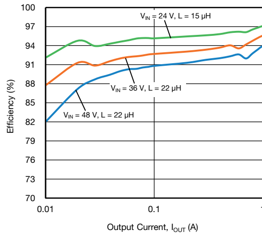
Fig. 27 - SiC473 Efficiency vs. Output Current - Light Load, VOUT = 12 V
