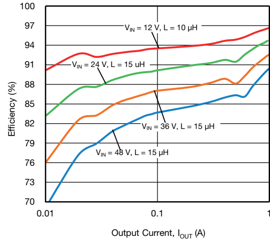
Fig. 26 - SiC473 Efficiency vs. Output Current - Light Load, VOUT = 5 V
