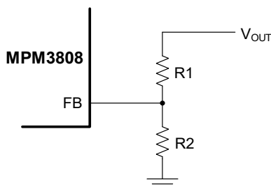
Figure 1: Feedback Divider Network with Adjustable Output
