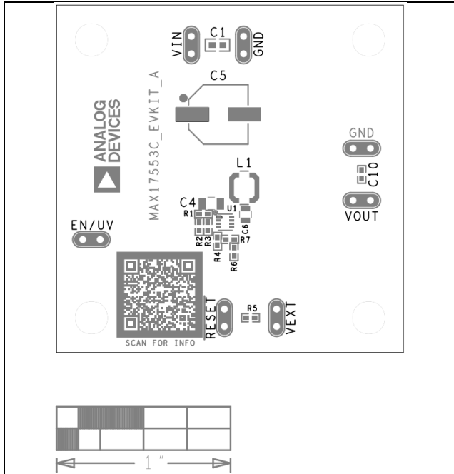
MAX17553C EV Kit PCB Layout—Top Silkscreen
