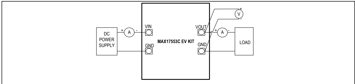
Figure 1. MAX17553C EV Kit Setup Diagram
