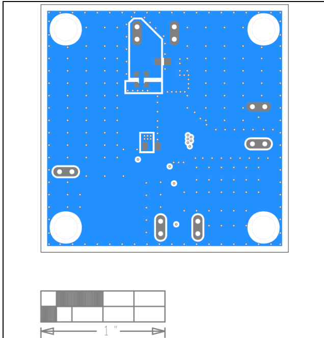
MAX17553C EV Kit PCB Layout—Bottom Layer
