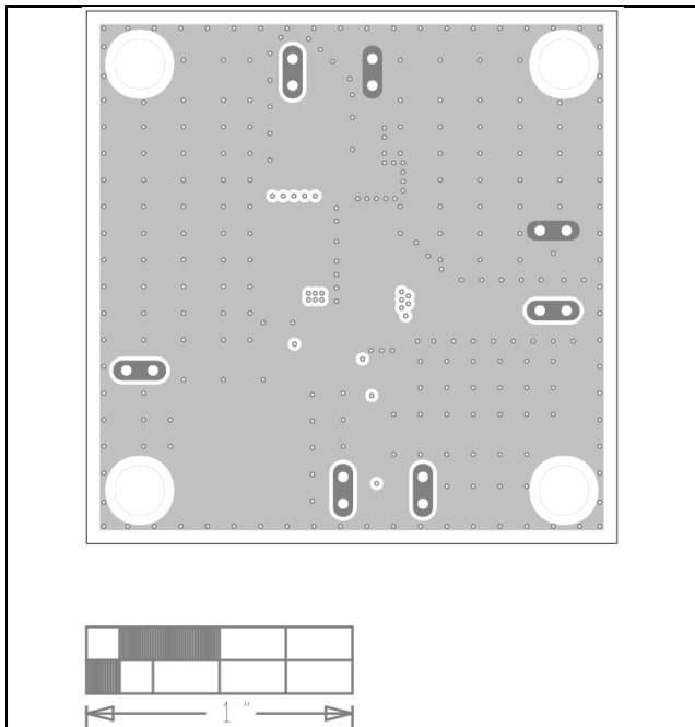
MAX17553C EV Kit PCB Layout—Layer 2
