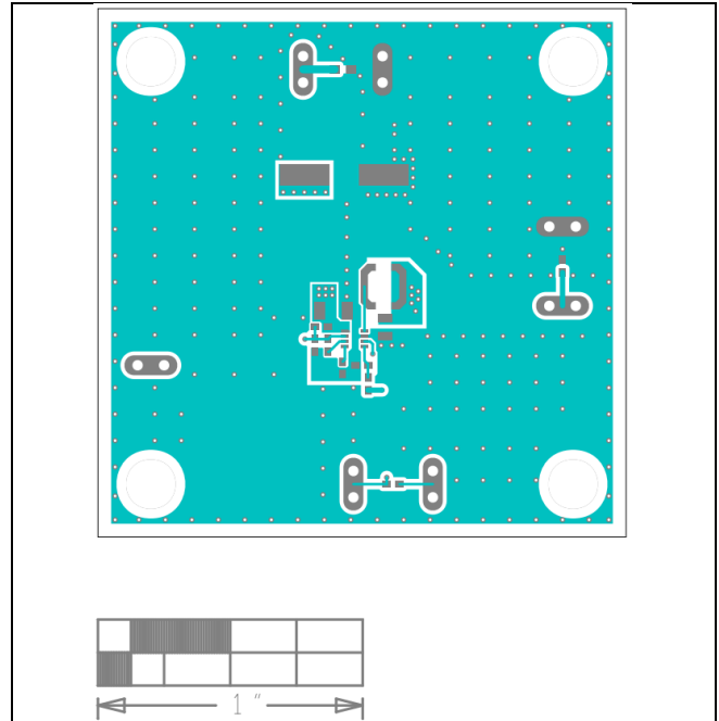
MAX17553C EV Kit PCB Layout—Top Layer
