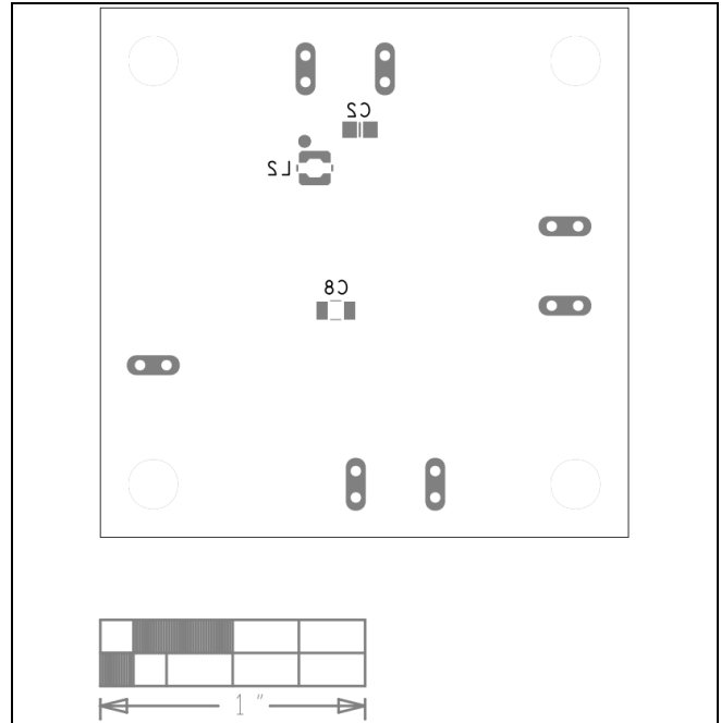
MAX17553C EV Kit PCB Layout—Bottom Silkscreen
