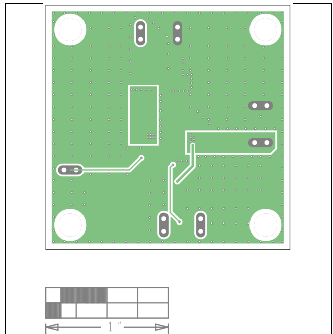
MAX17553C EV Kit PCB Layout—Layer 3
