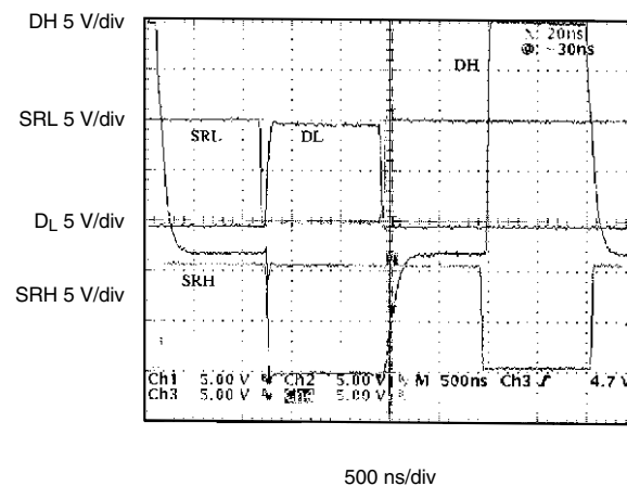
Figure 12. Drive Waveforms
