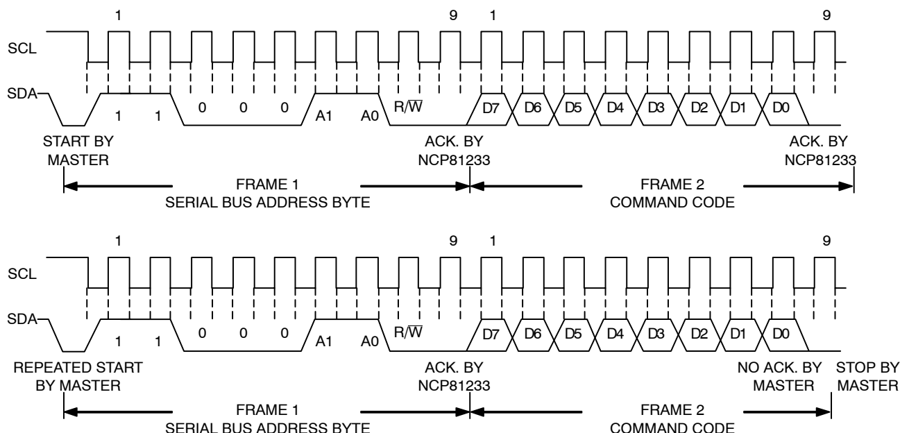
Figure 21. Read Byte
