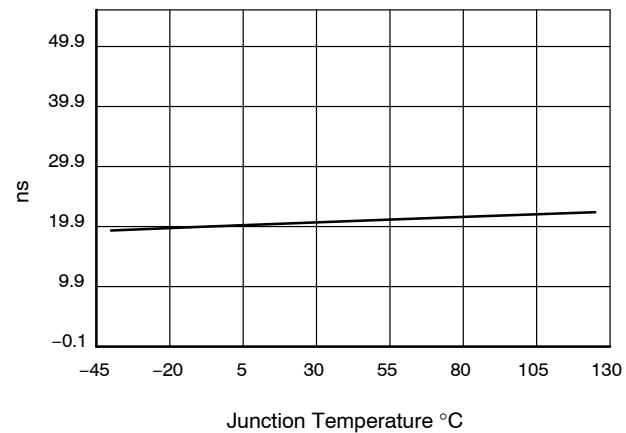
t_{ILIM(DELAY)}
