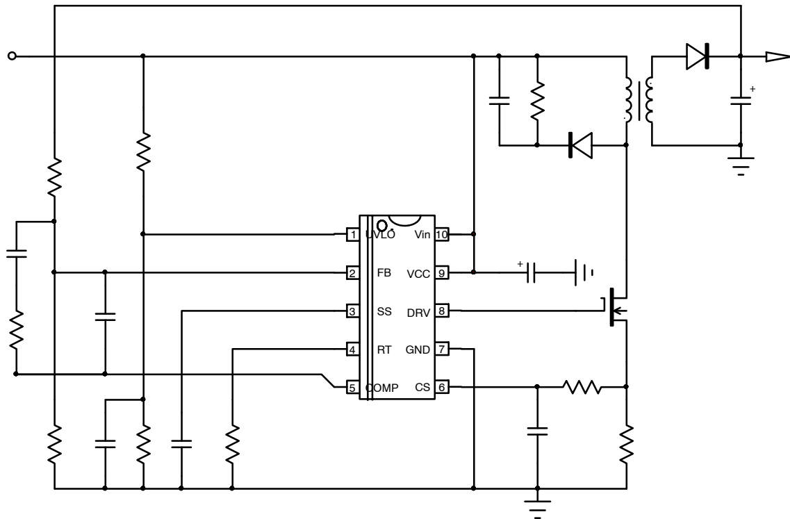
Figure 1. Low-Dissipation Wide-Range Application Non-Isolated Converter
