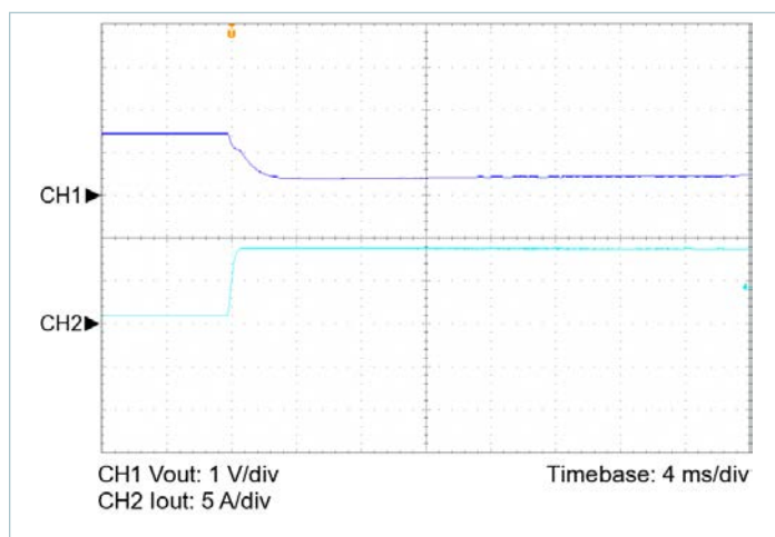
Figure 8 — 10 – 100% load transient response, V_{IN} = 100\text{V} , nominal trim, C_{OUT\_EXT} = 1000\mu\text{F}
