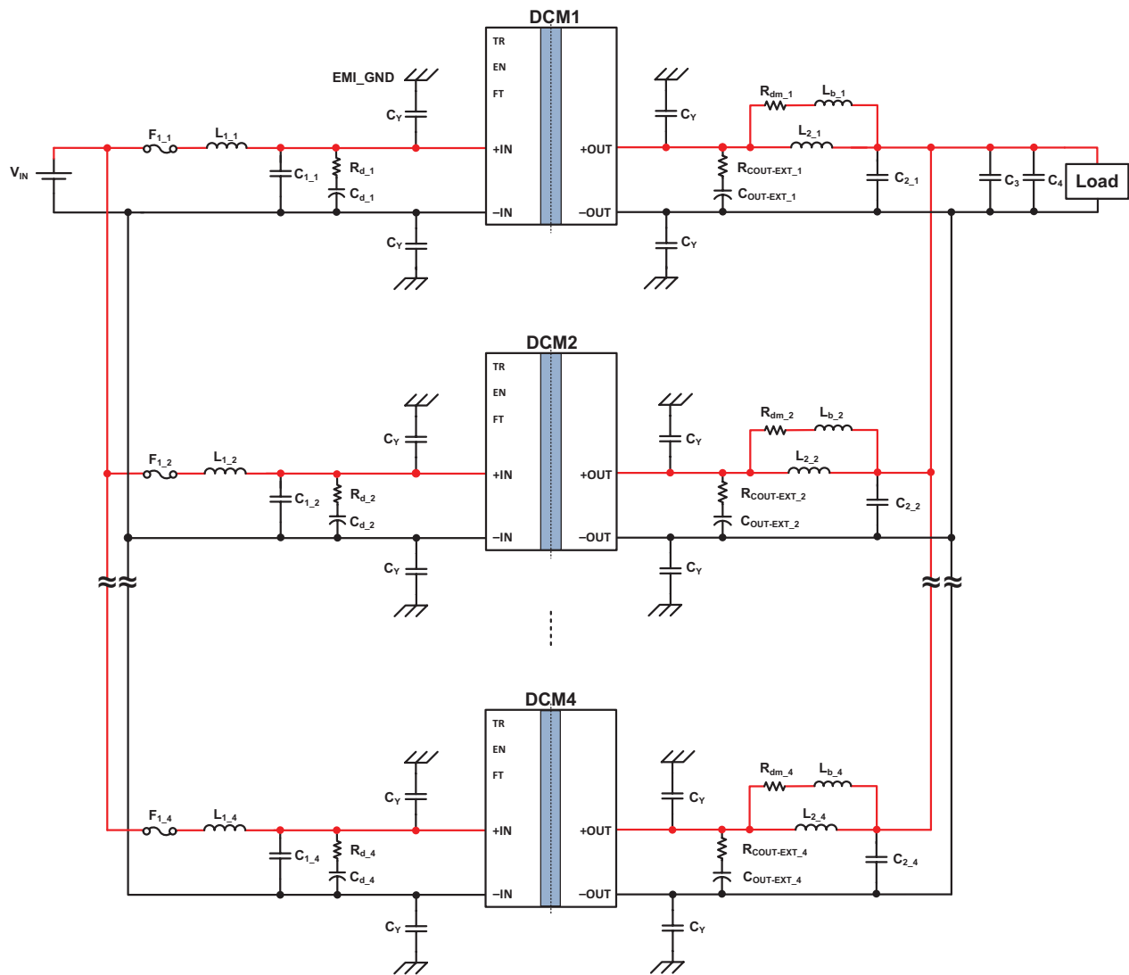
Typical application 1: DCM3623xA5N31B4yzz in an array of four units
