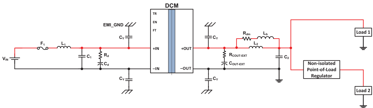
Typical application 2: single DCM3623xA5N31B4yzz, to a non-isolated regulator, and direct to load
