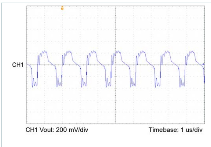
Figure 22 — Output voltage ripple, V_{IN} = 100\text{V} , V_{OUT} = 28.0\text{V} , C_{OUT\_EXT} = 1000\mu\text{F} , R_{LOAD} = 3.256\Omega
