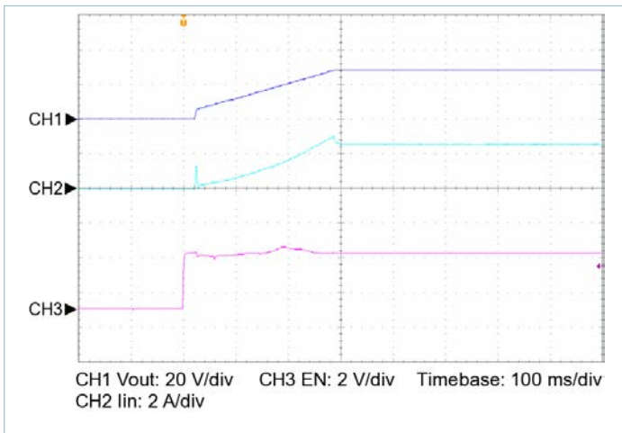
Figure 20 — Start up from EN, V_{IN} = 100\text{V} , C_{OUT\_EXT} = 20000\mu\text{F} , R_{LOAD} = 3.256\Omega
