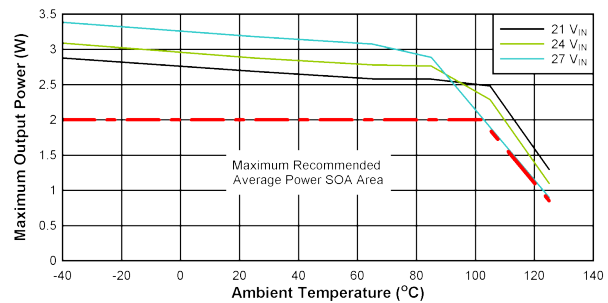
Figure 10-2. SOA Derating Curves: V_{D\bar{D}-V\bar{E}E} = 18\text{ V} , V_{C\bar{O}M-V\bar{E}E} = 5\text{ V} , T_{shut}=150^\circ\text{C} , No Load on V_{C\bar{O}M-V\bar{E}E} .
