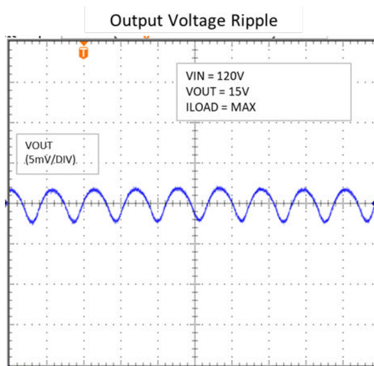
Figure 7-4. Output Voltage Ripple
