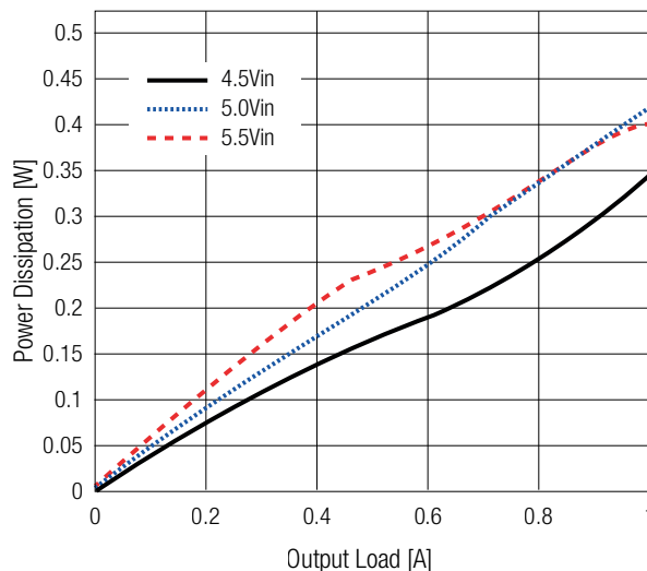
Power Dissipation
