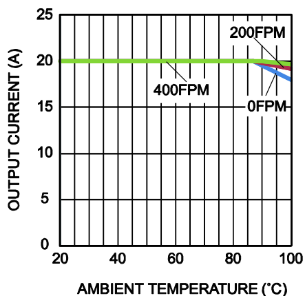
Output Current De-Rating 12V to 1.2V, 600kHz
