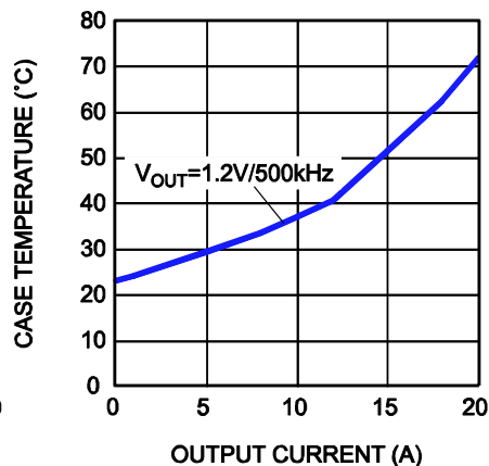
Thermal Results T_{ambient}=22^{\circ}C
