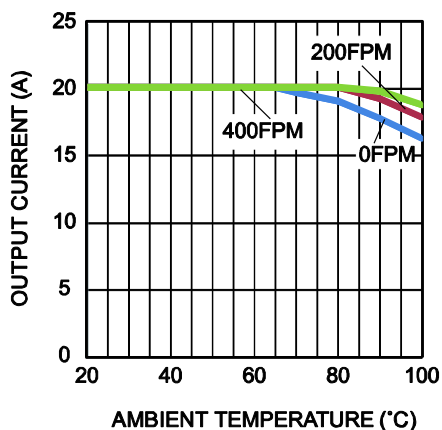
Output Current De-Rating 12V to 2.5V, 600kHz
