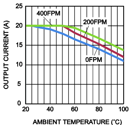
Output Current De-Rating 12V to 5V, 600kHz
