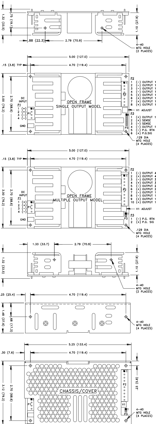
ALL DIMENSIONS IN INCHES (mm)
