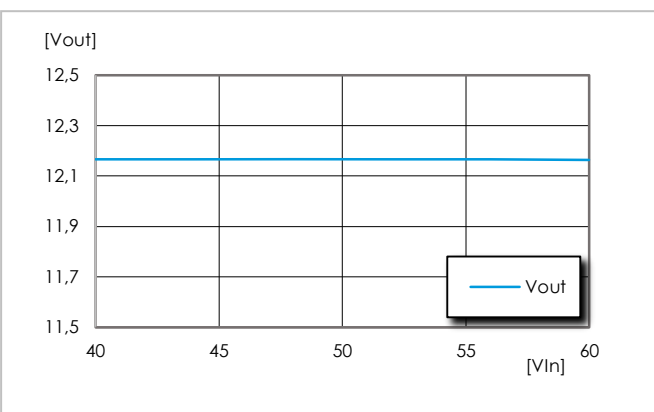
Output voltage vs. input voltage at T_{P1} = +90^{\circ}C
