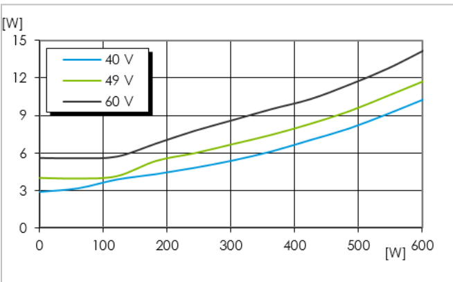
Dissipated power vs. output power and input voltage at T_{P1} = +90^{\circ}C
