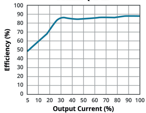
EFFICIENCY VS OUTPUT LOAD ( V_{in} = 24V ) PYBE30-Q24-S5
