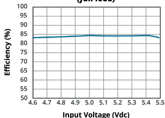
EFFICIENCY VS INPUT VOLTAGE PESE2-S5-S5-M (full load)
