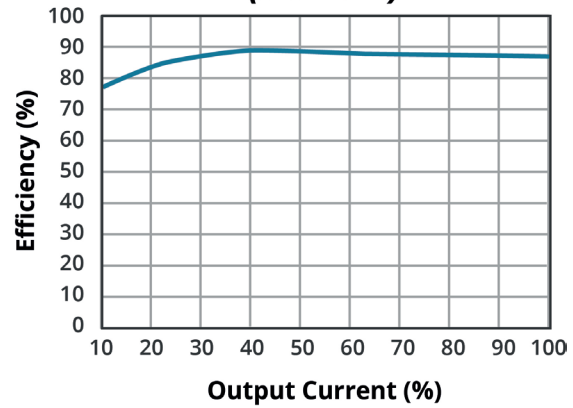
EFFICIENCY VS OUTPUT LOAD PDSE2-S24-S5-M ( V_{in} = 24\text{ V} )
