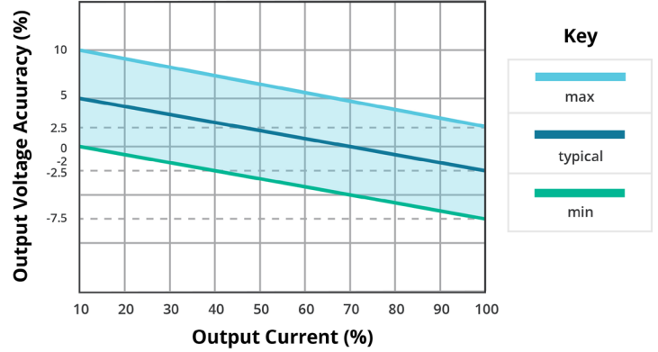
OUTPUT REGULATION CURVE 3.3, 5 Vdc input model / 5, 9, 12, 15, 24 Vdc output models (nominal input)
