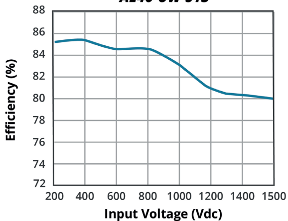
EFFICIENCY VS INPUT VOLTAGE AE40-UW-S15
