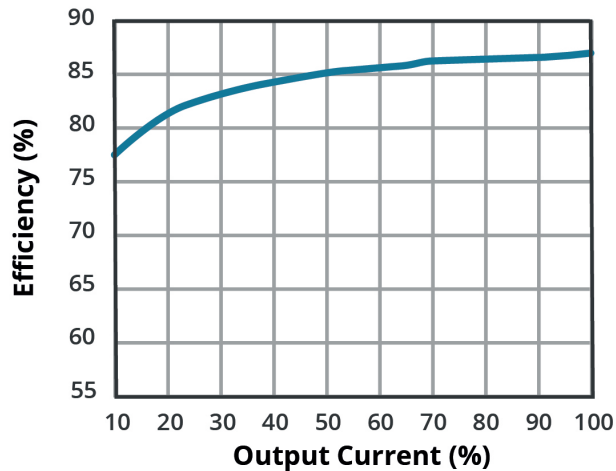
EFFICIENCY VS OUTPUT LOAD AE40-EW-S24-T
