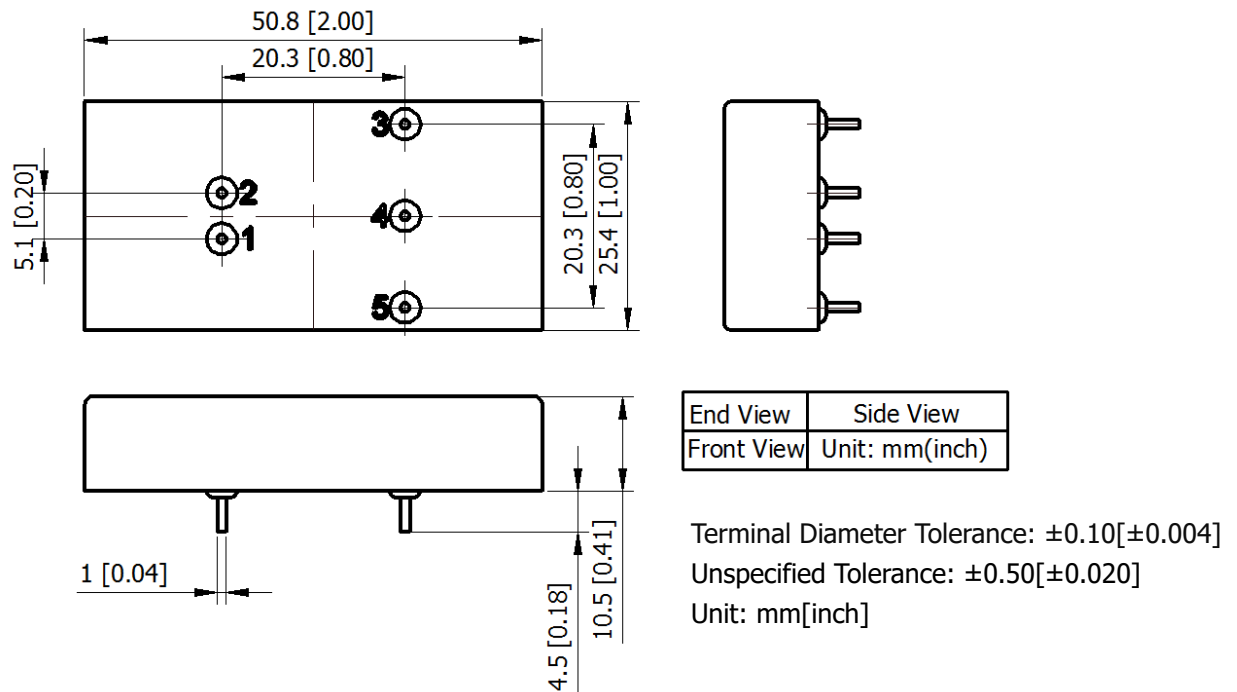
Figure 7. Outline Dimensions
