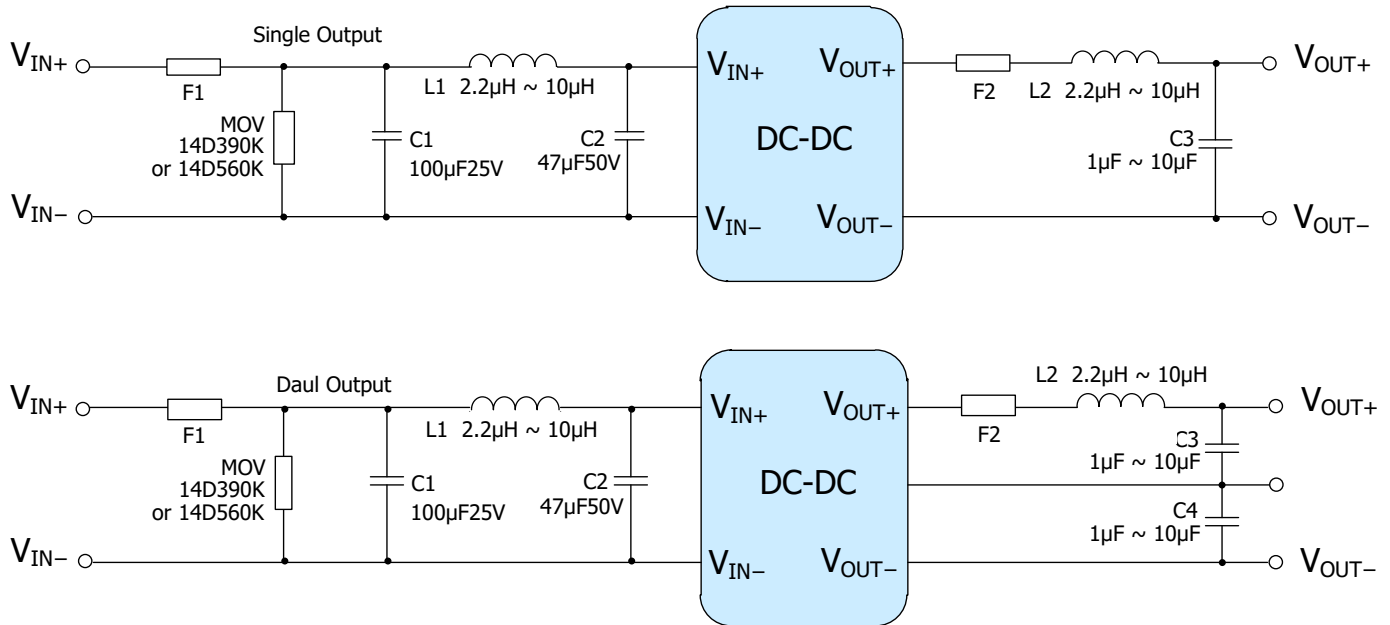
Figure 6. Typical Applications
