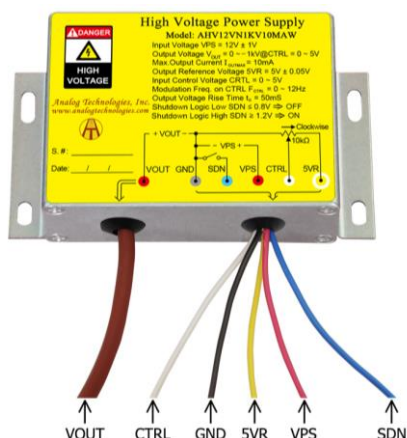
Figure 2. The Connecting Lead Wires of AHV12VN1KV1MAW
