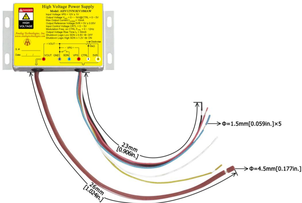
Figure 13. Connecting Lead Wires of AHV12VN1KV10MAW
