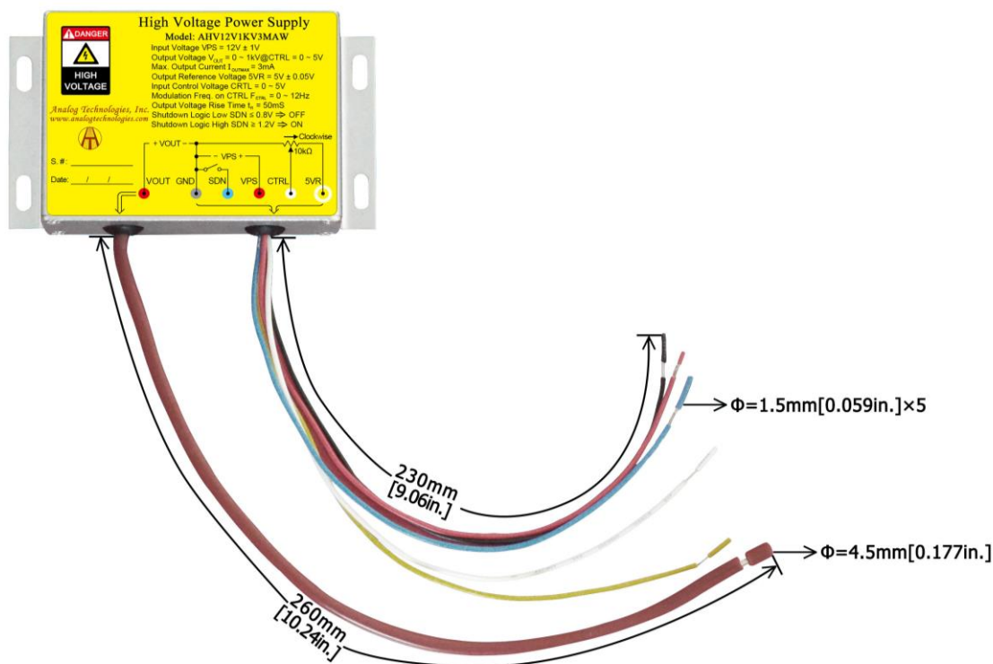
Figure 13. Connecting Lead Wires of AHV12V1KV3MAW
