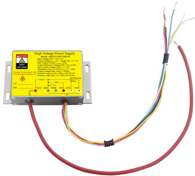
Figure 1.1. Top View of AHV12V1KV2MAW
