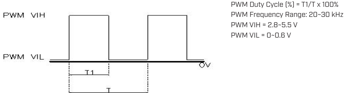
Figure 3: PWM Input Signal
