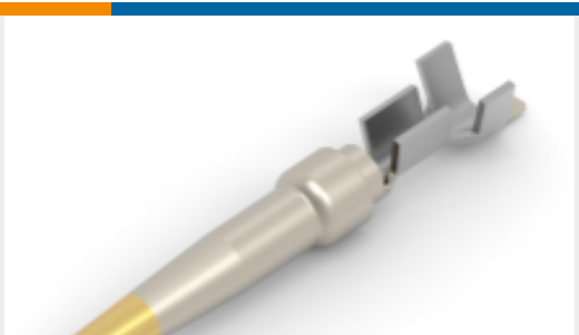
TE Part #66505-9 D-Sub Conn Contacts: Socket, Phosphor Bronze, Signal, Size 20
